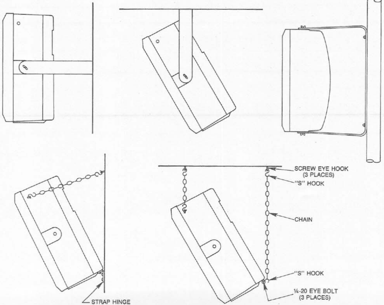
FIGURE 8 — Mounting Variations
